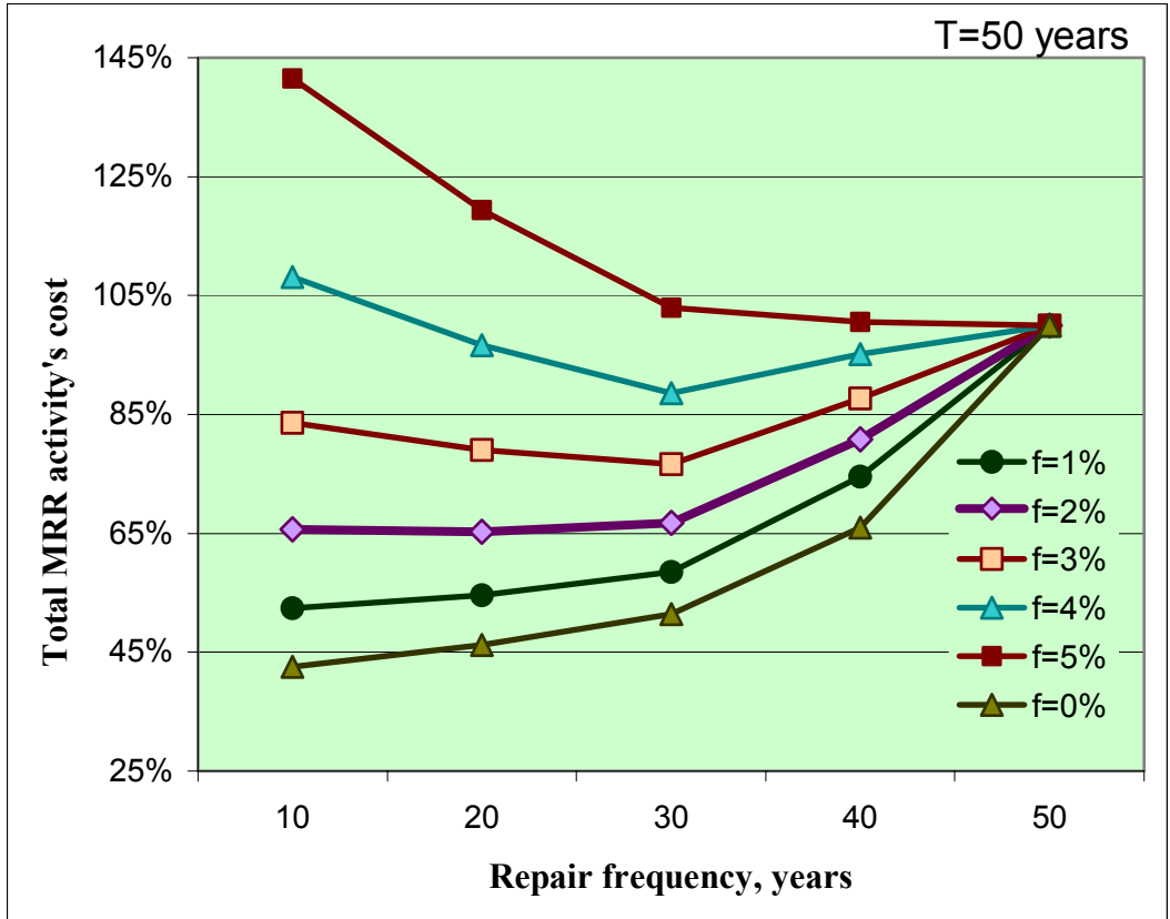
FIGURE 8 Total MRR activity cost depends on repair frequency and discount rate (f)
