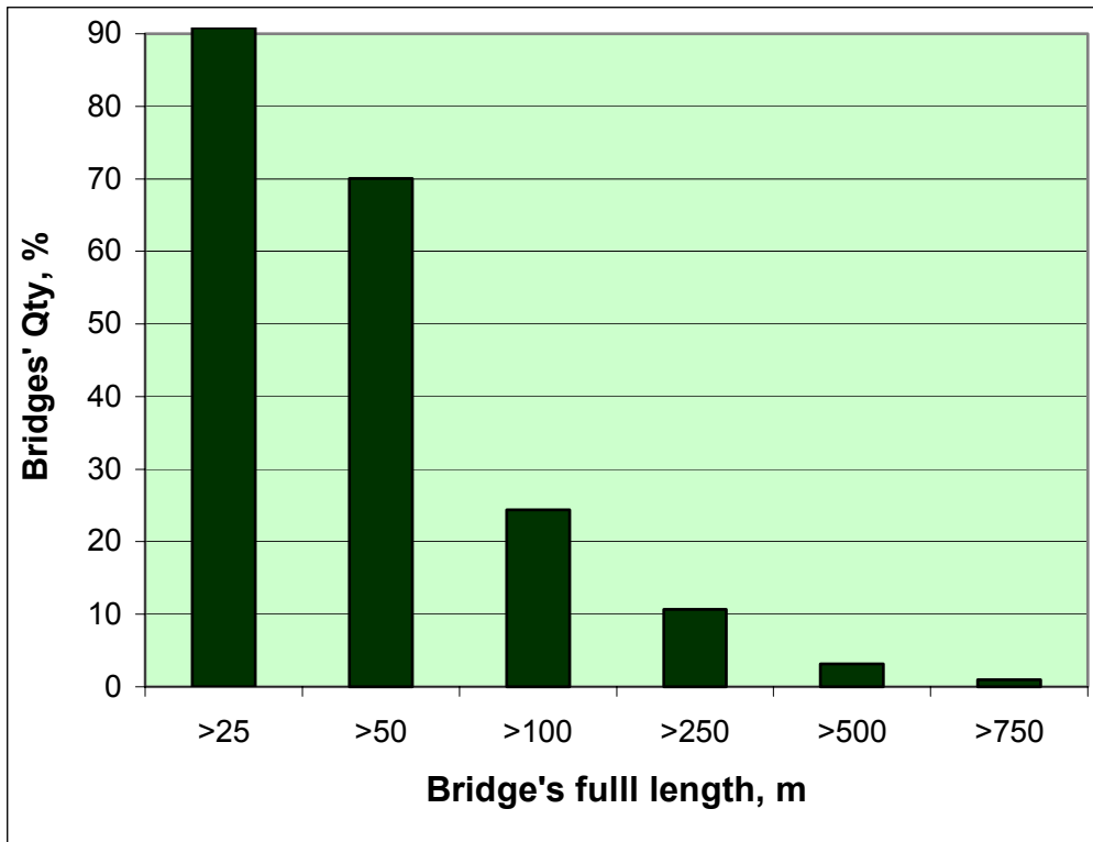
FIGURE 1b Moscow Bridge stock. Distribution of structures by size
