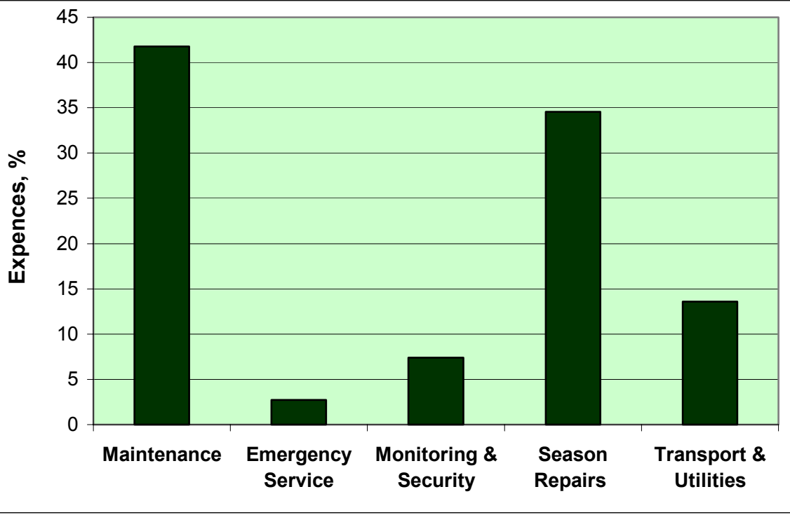
FIGURE 2 Moscow Bridge stock. Expenses for structures' routine care.
