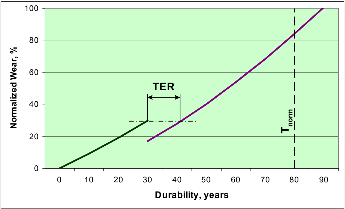
FIGURE 6 Deterioration model for SSE ID #6000 “Reinforced Concrete Beam” modified because of SRP ID #1021 “Injection” application
